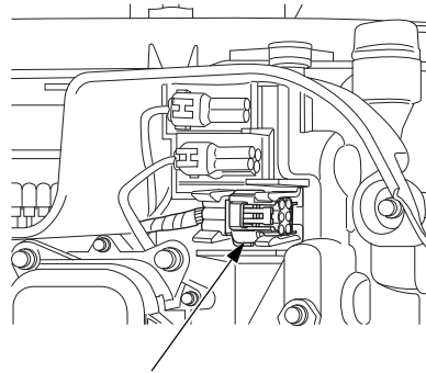
NMEA-INTERFACE-STECKER
